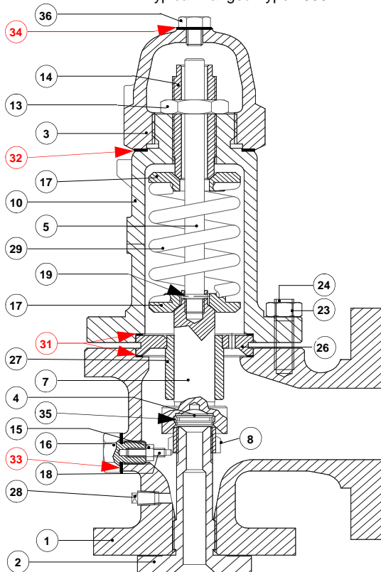
Typical Flanged Type 2500
