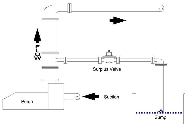
Typical Installation
