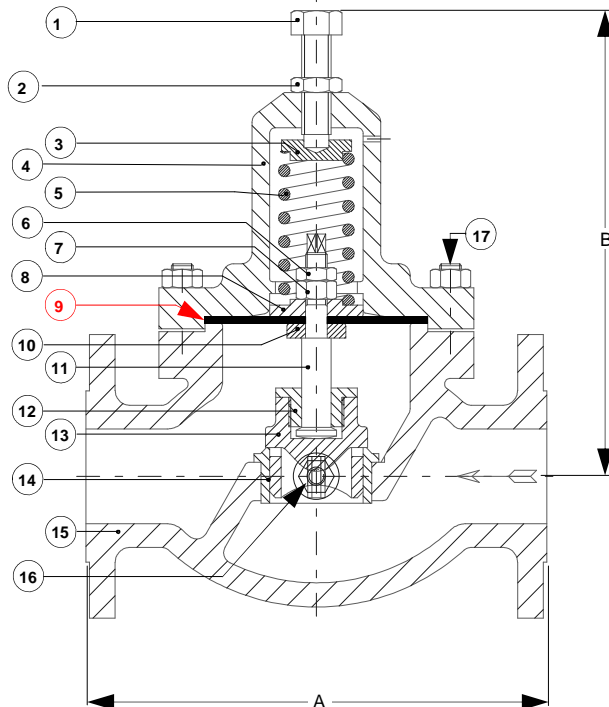
Typical Carbon Steel Type 9
